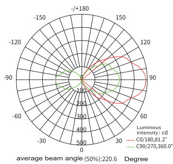
Light distribution curve of indoor light
