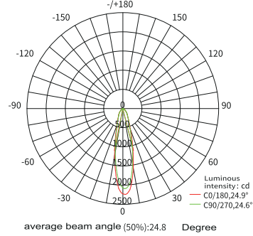
Light distribution curve of indoor light
