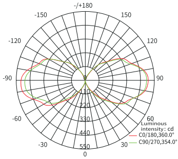
Light distribution curve of indoor light
