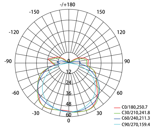
AVERAGE BEAM ANGLE (50%): 216 DEG.
