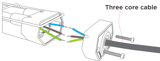
Schematic diagram of cable installation
